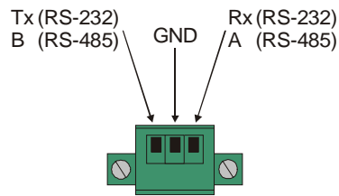
Figure 2-1: Serial Interface
