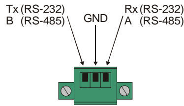
Figure 3: Serial Interface
