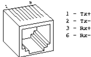
Figure 2: Network Interface
